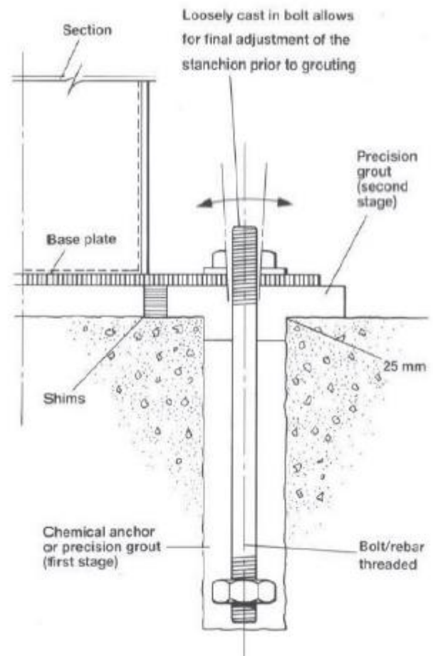
Typical detail of stanchion base plate
